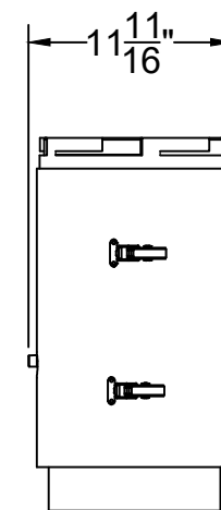
Rear View
