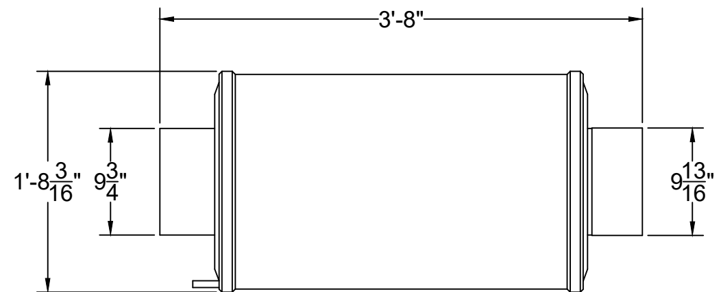
Side View
