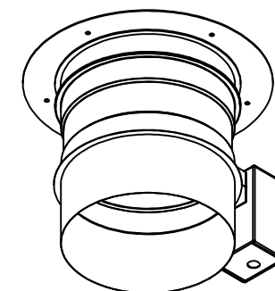
Isometric (Bottom)
