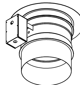
Isometric (Bottom)
